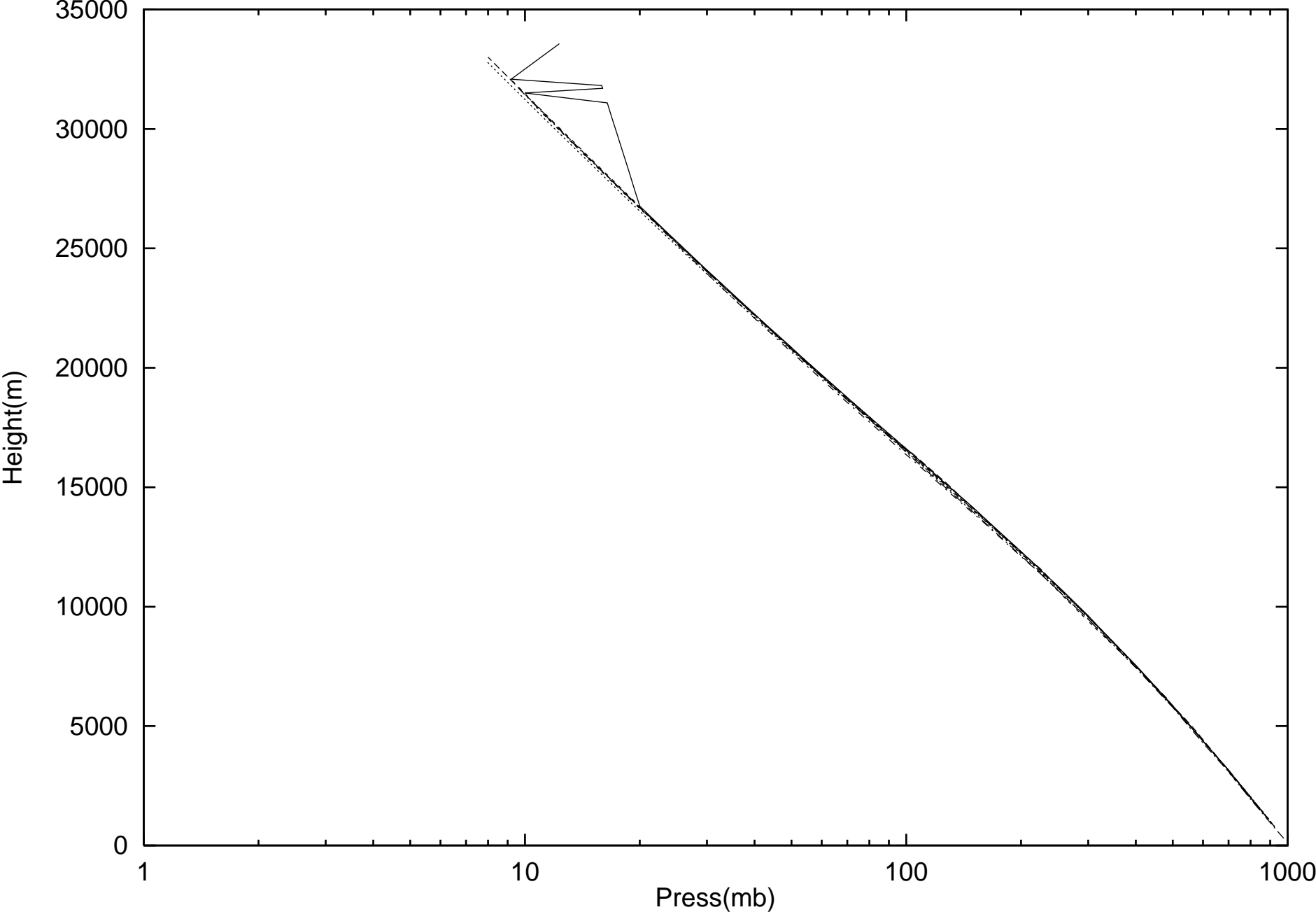
Firex 1994 - Sonde - 16/00
