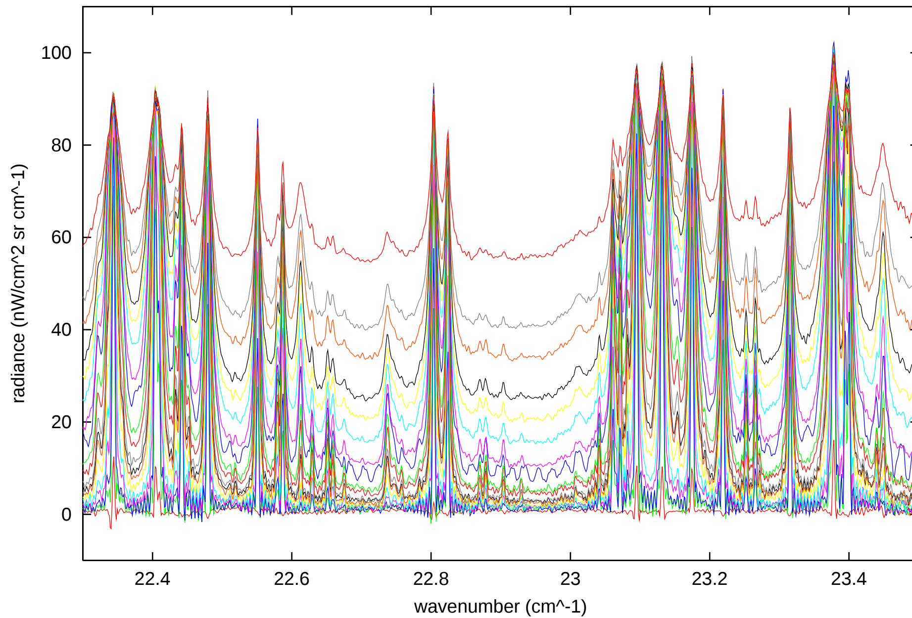
Sequence 181 199
