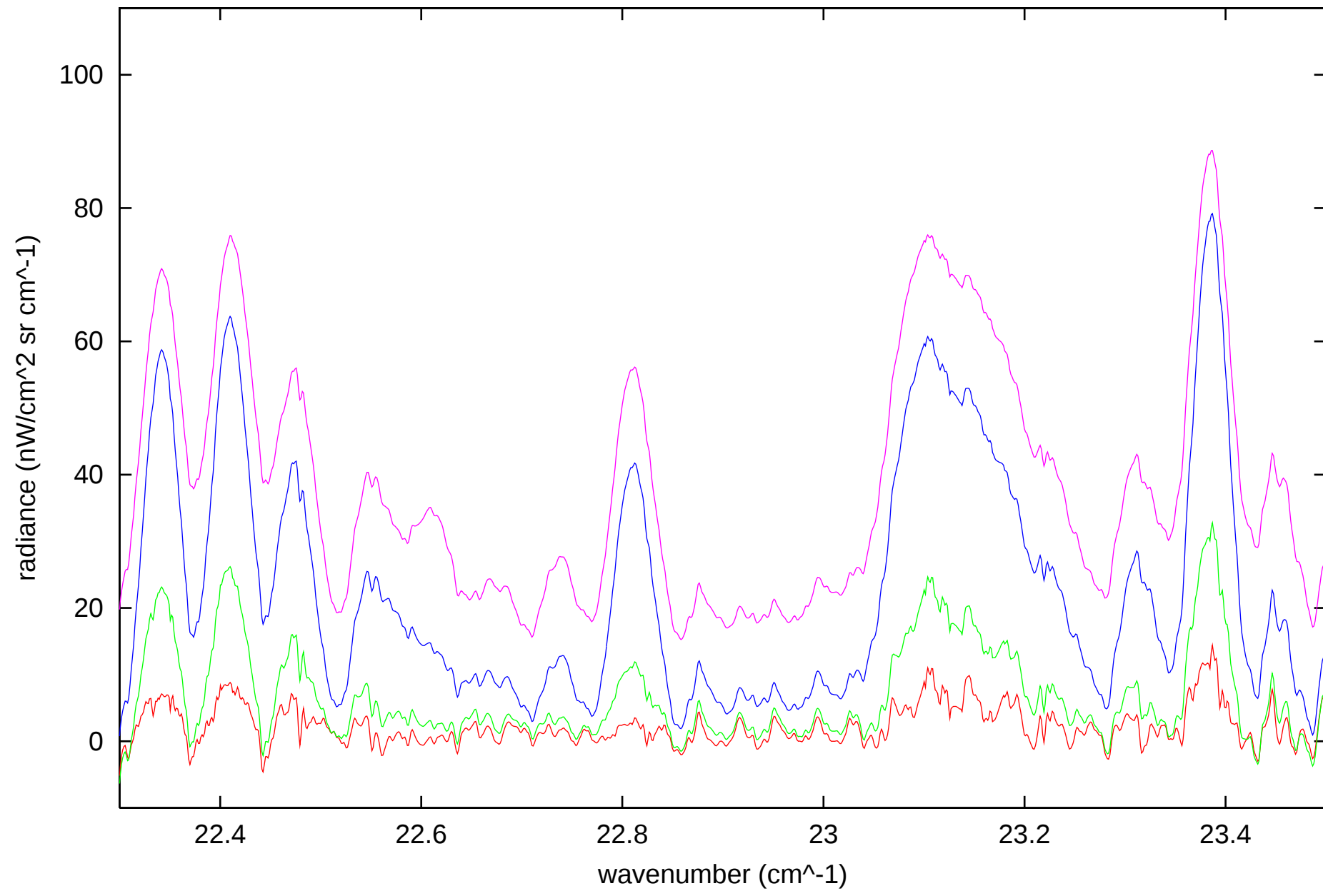
Sequence 94 97
